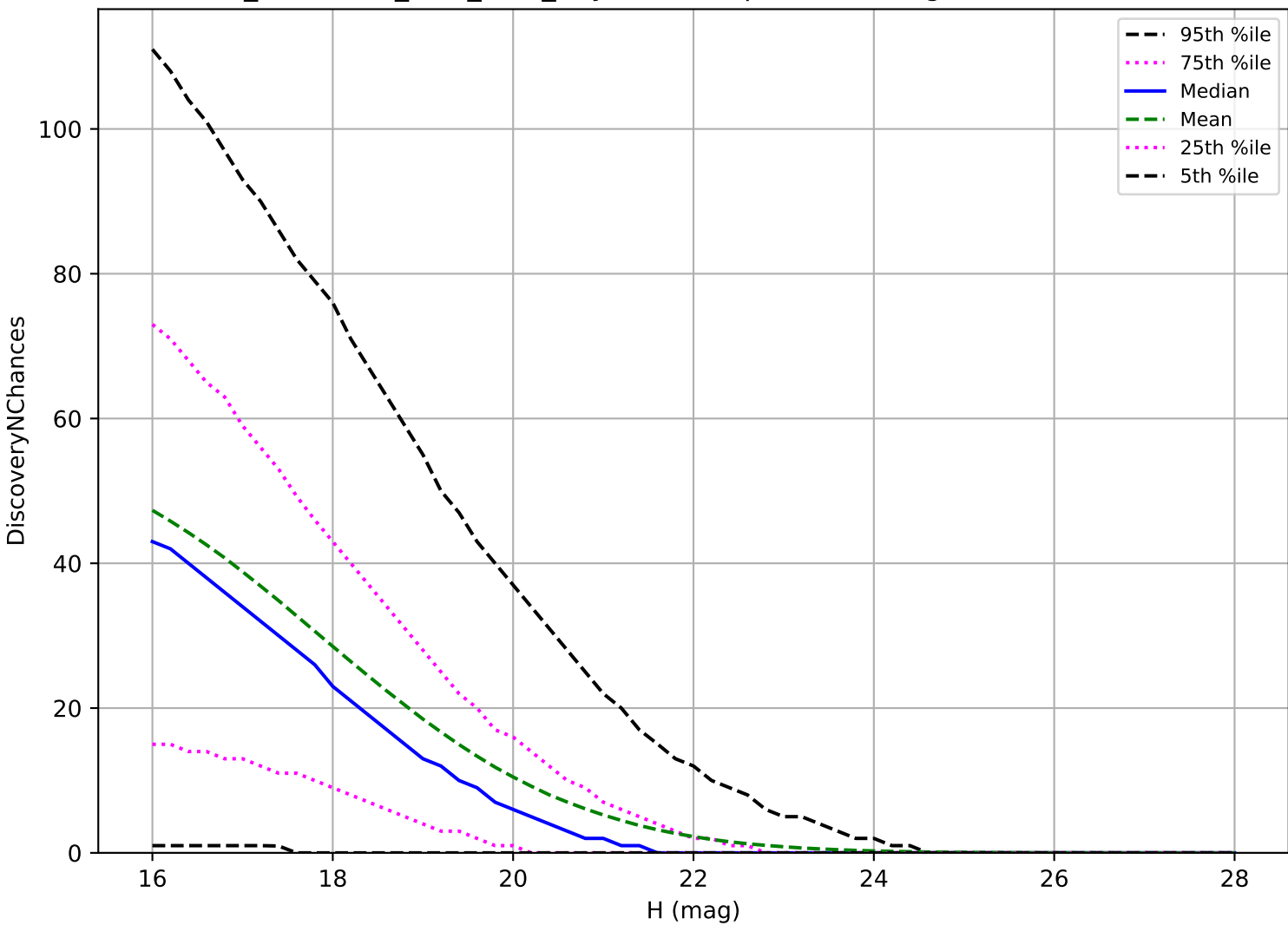
too_combined_s2.0_v3.4_10yrs: PHA 3 pairs in 15 nights detection loss
