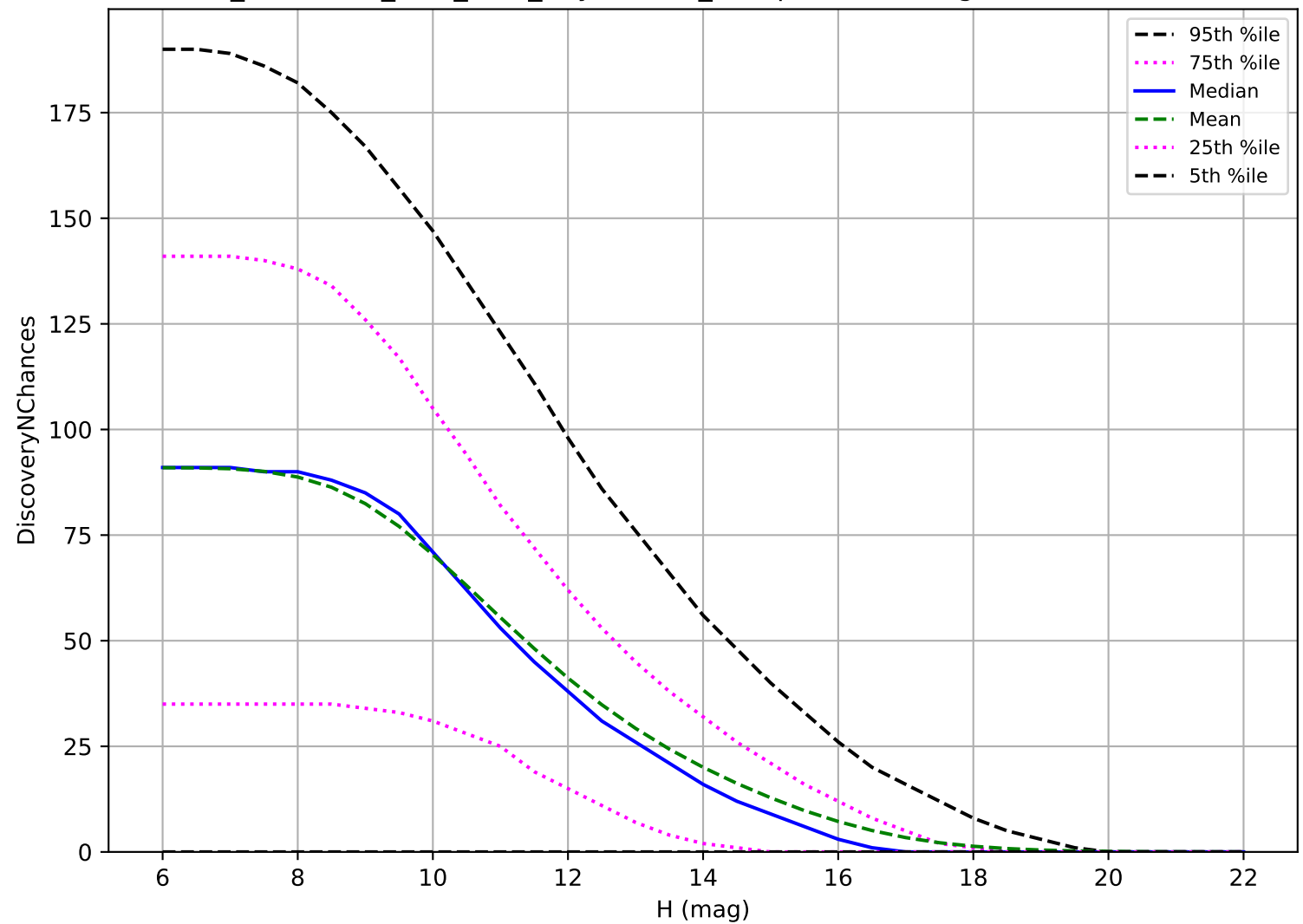
too_combined_s2.0_v3.4_10yrs: OCC_r5 3 pairs in 15 nights detection loss
