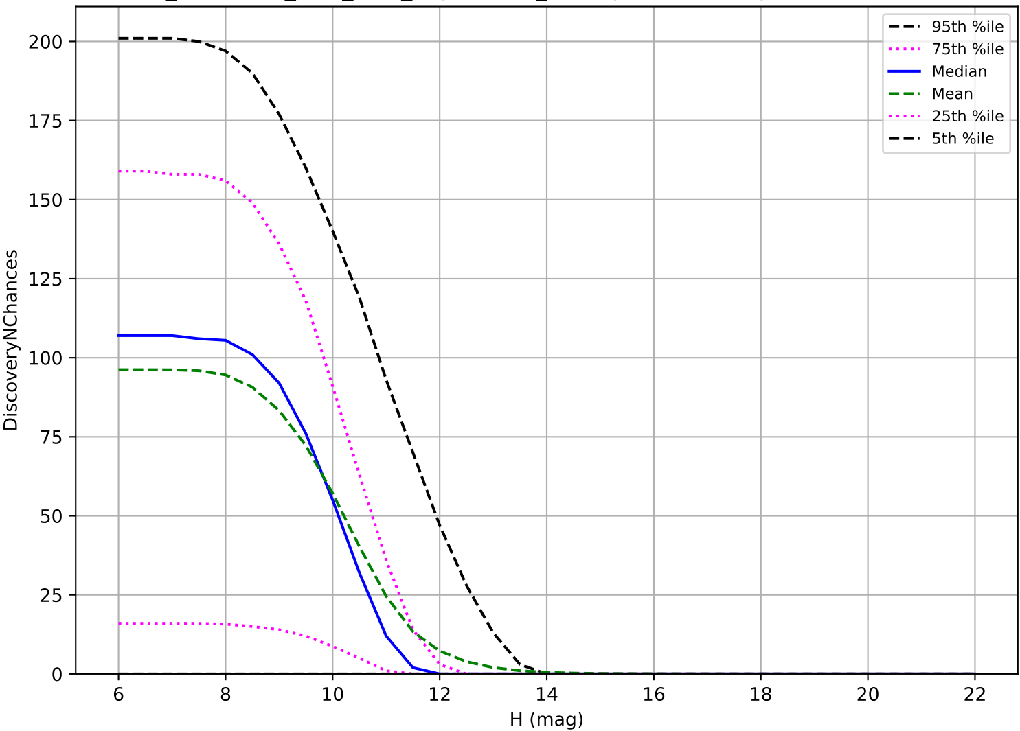
too_combined_s2.0_v3.4_10yrs: OCC_r20 3 pairs in 15 nights detection loss
