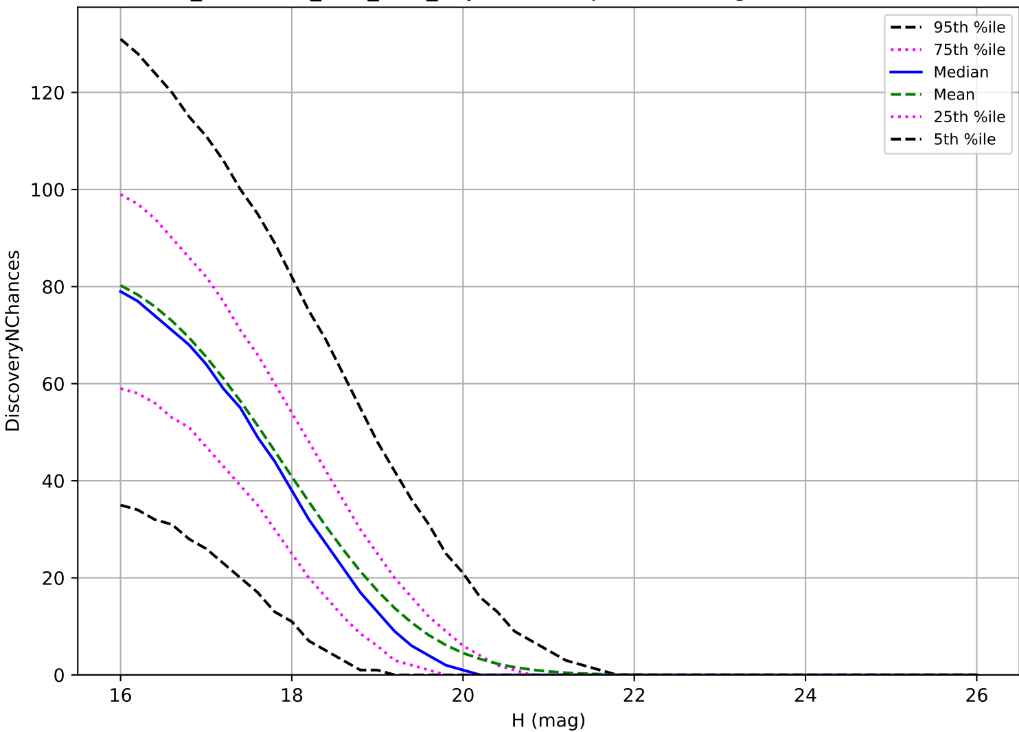
too_combined_s2.0_v3.4_10yrs: MBA 3 pairs in 15 nights detection loss
