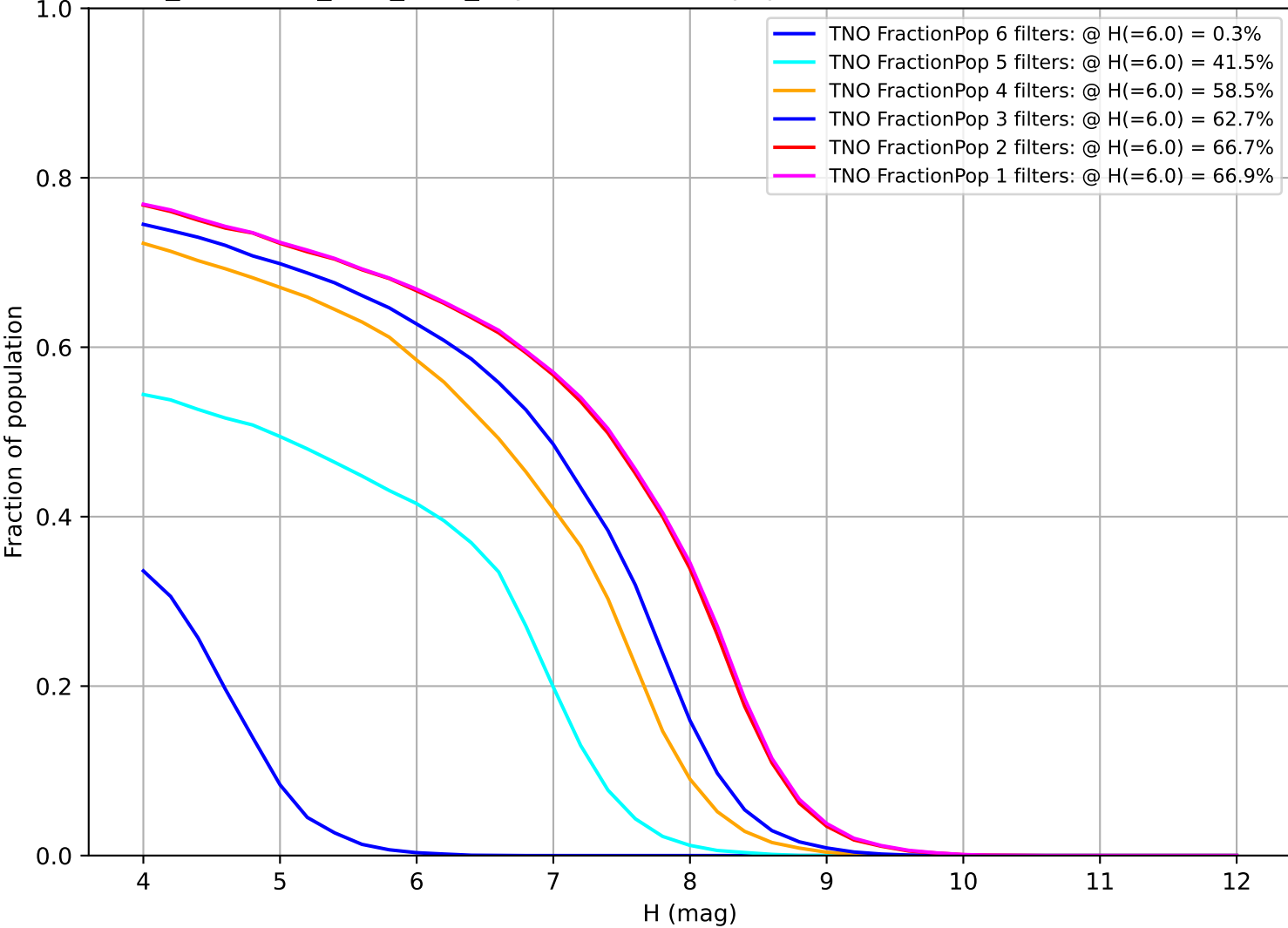
too_combined_s2.0_v3.4_10yrs: Fraction of population with colors in X filters TNO
