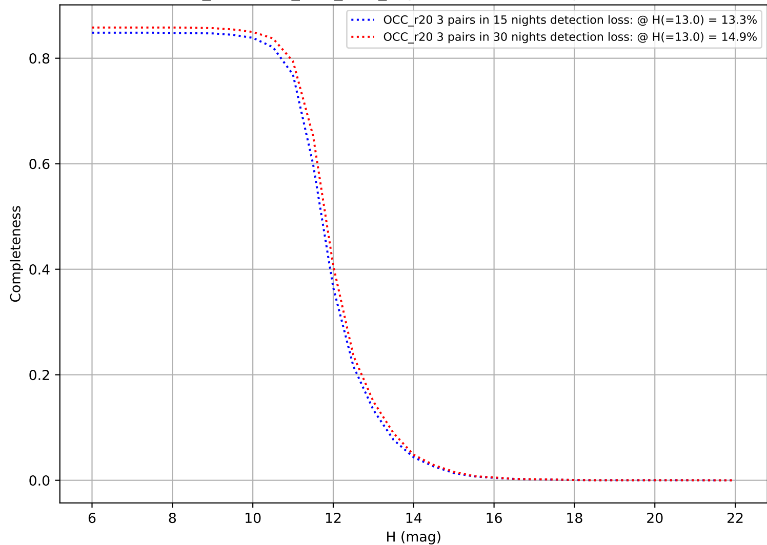
too_combined_s2.0_v3.4_10yrs: DifferentialCompleteness
