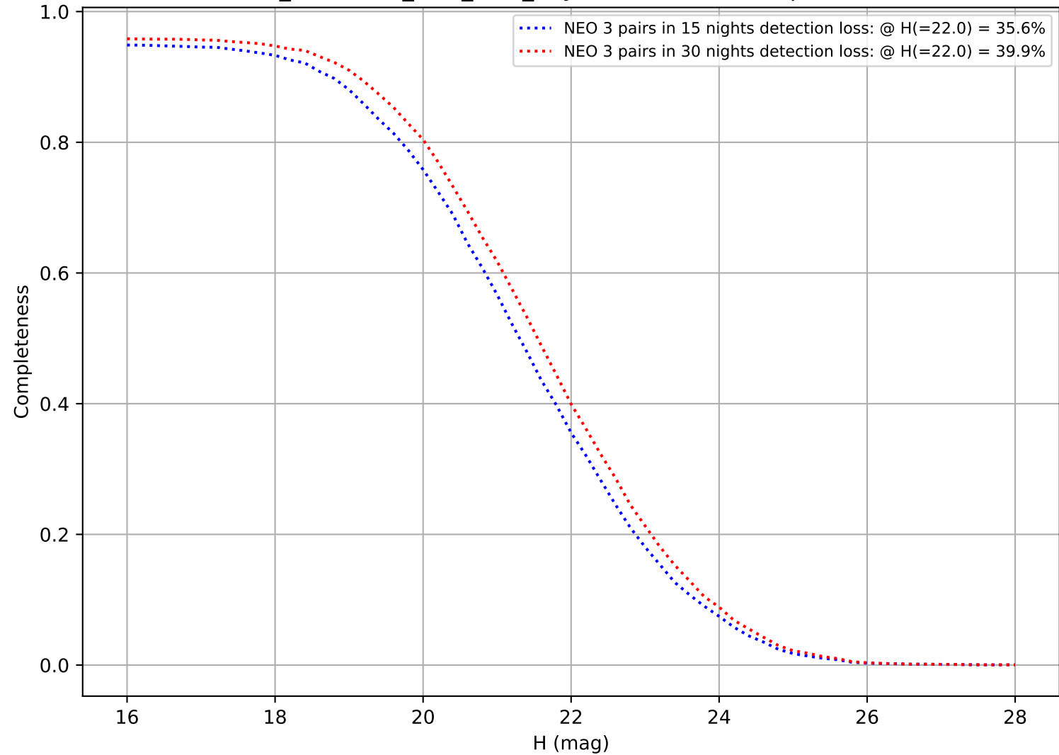
too_combined_s2.0_v3.4_10yrs: DifferentialCompleteness
