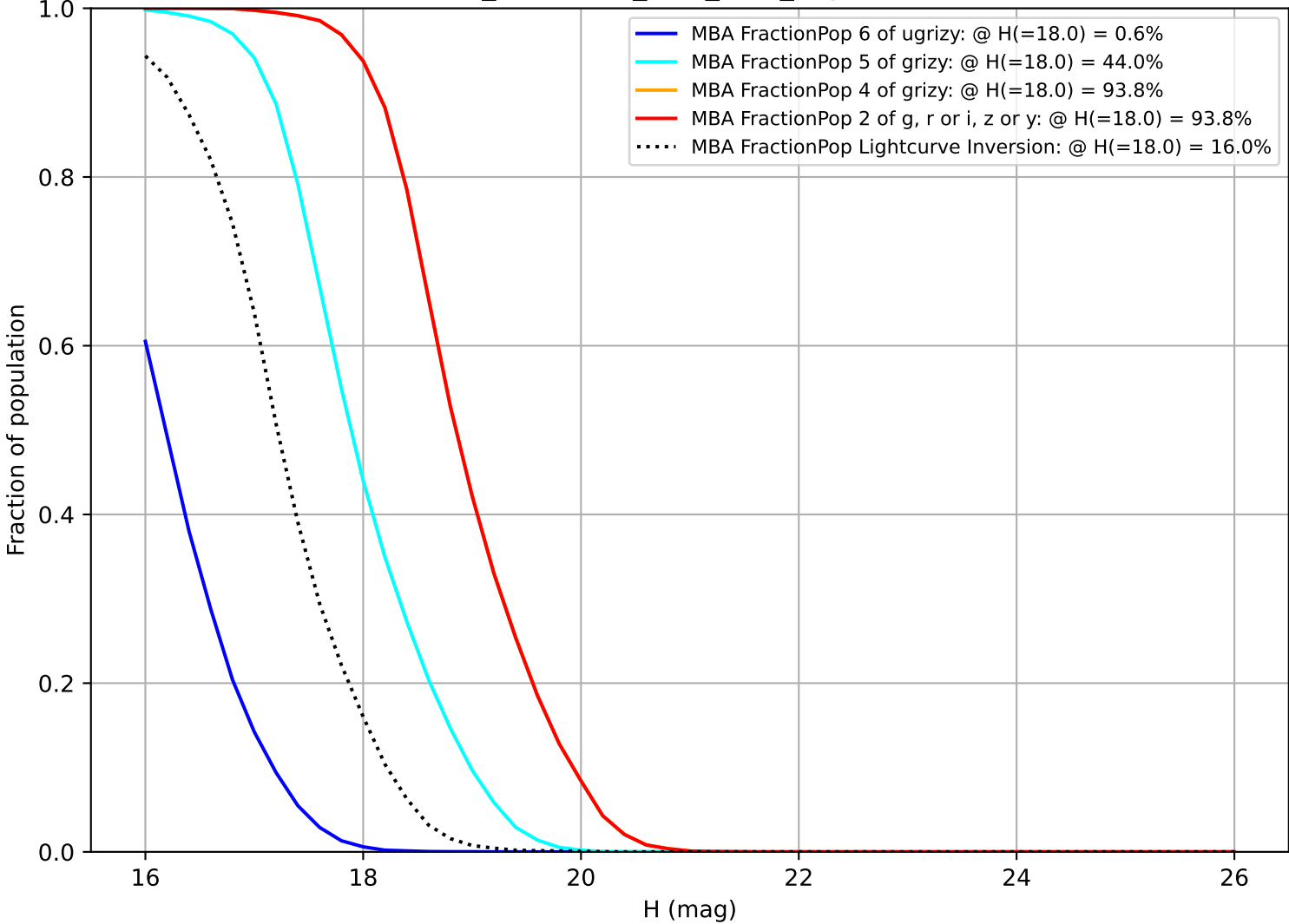
too_combined_s2.0_v3.4_10yrs MBA
