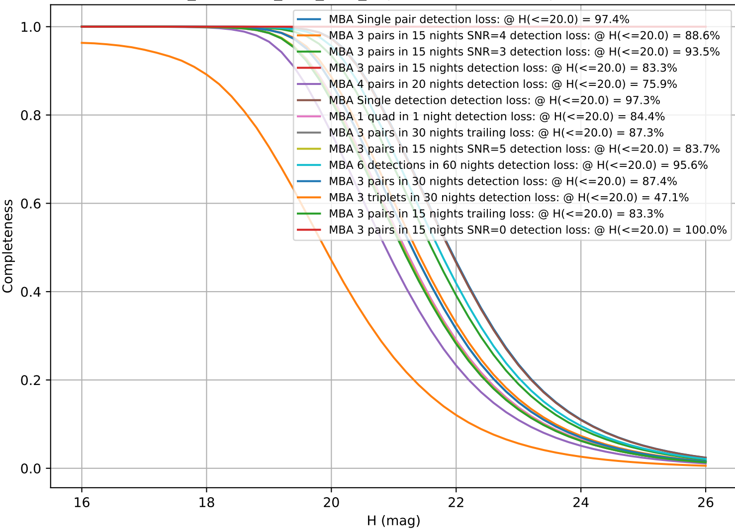
too_combined_s2.0_v3.4_10yrs: CumulativeCompleteness
