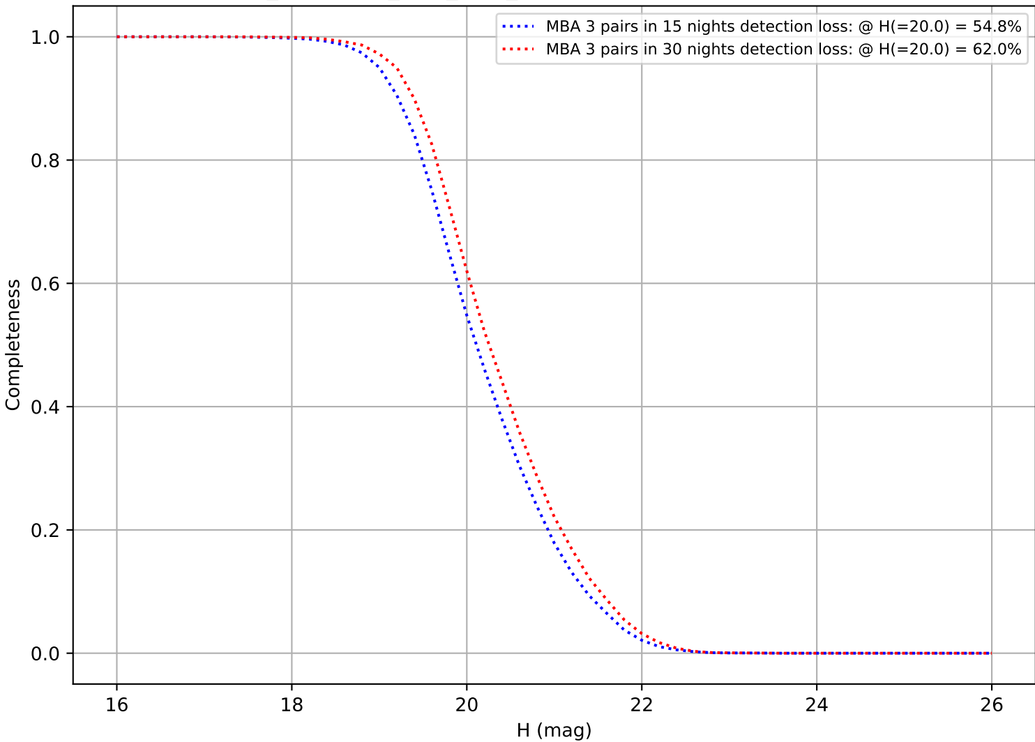
too_combined_s2.0_v3.4_10yrs: DifferentialCompleteness
