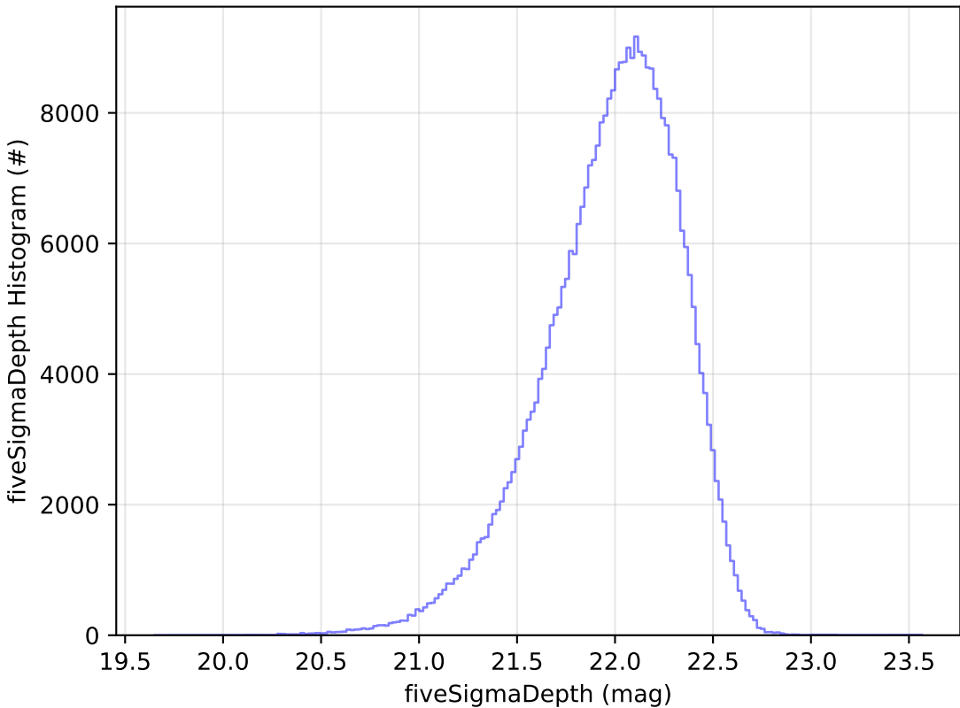
too_combined_s2.0_v3.4_10yrs y: fiveSigmaDepth Histogram
