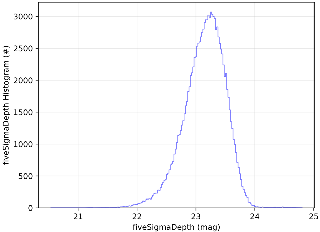
too_combined_s2.0_v3.4_10yrs u: fiveSigmaDepth Histogram
