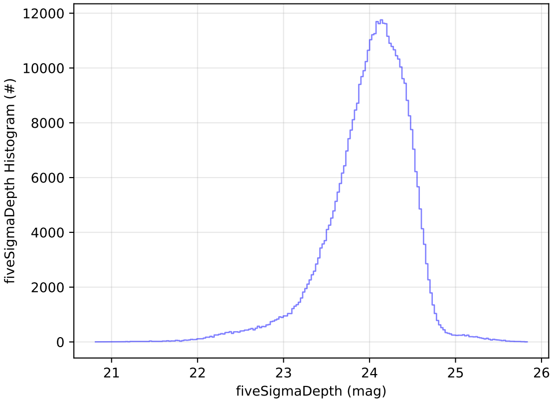
too_combined_s2.0_v3.4_10yrs r: fiveSigmaDepth Histogram
