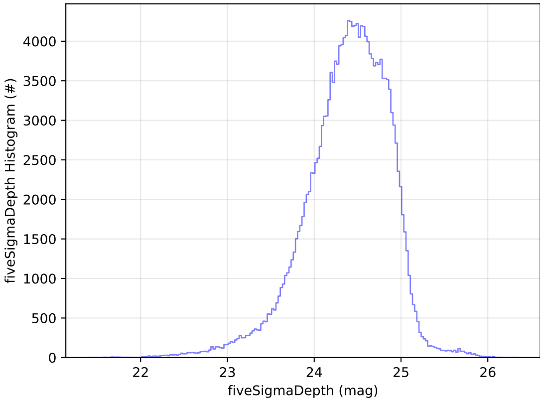
too_combined_s2.0_v3.4_10yrs g: fiveSigmaDepth Histogram
