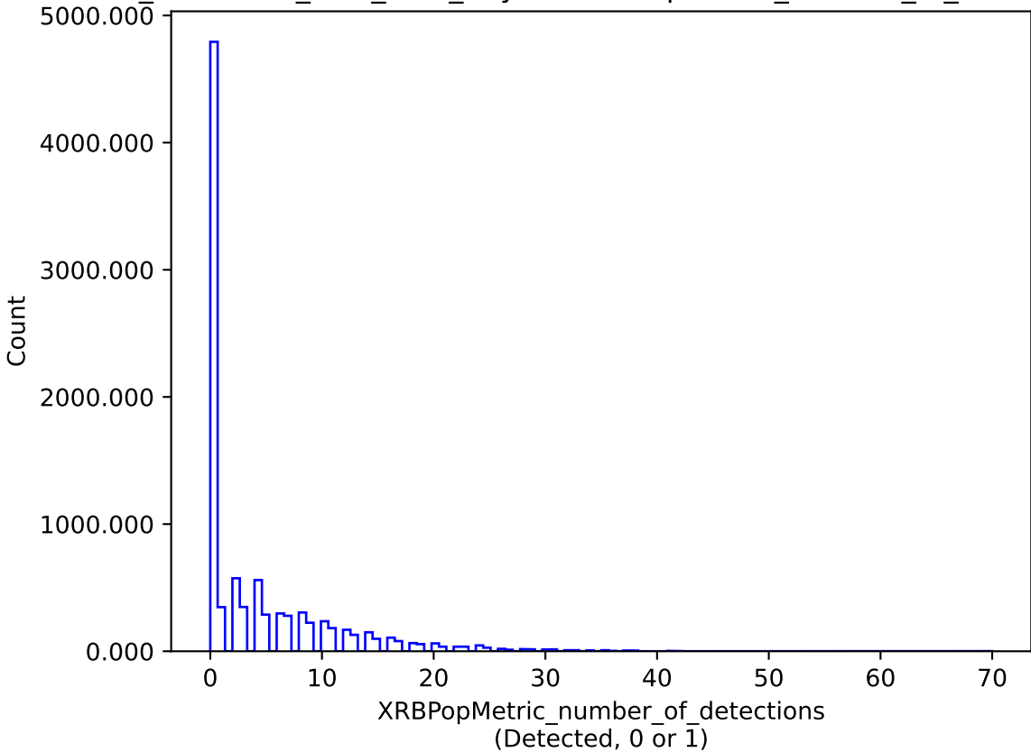
too_combined_s2.0_v3.4_10yrs : XRBPoMetric_number_of_detections
