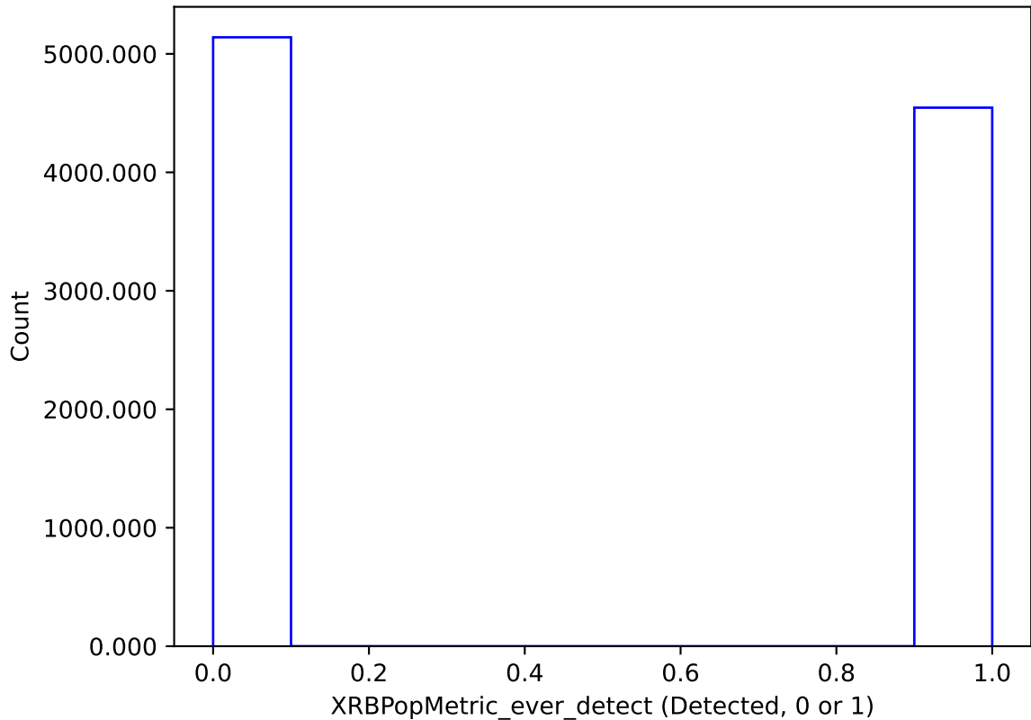
too_combined_s2.0_v3.4_10yrs : XRBPoMetric_ever_detect
