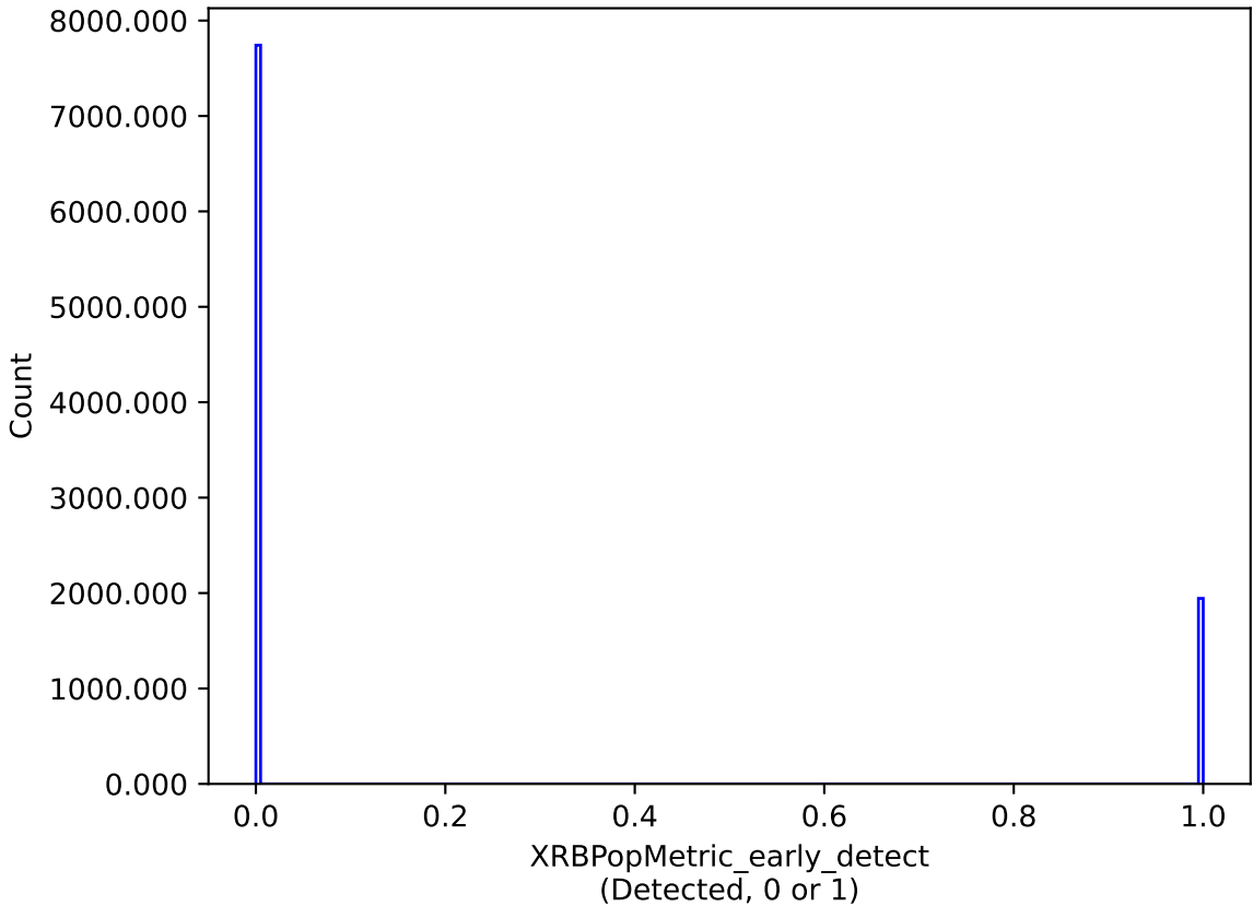
too_combined_s2.0_v3.4_10yrs : XRBPoMetric_early_detect
