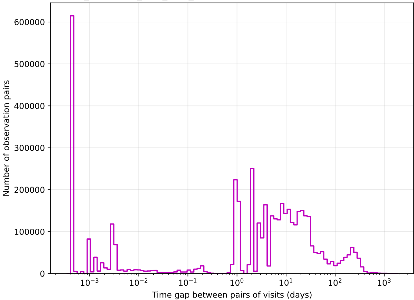
too_combined_s2.0_v3.4_10yrs z band: Tgaps observationStartMJD
