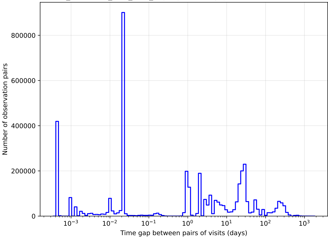
too_combined_s2.0_v3.4_10yrs y band: Tgaps observationStartMJD
