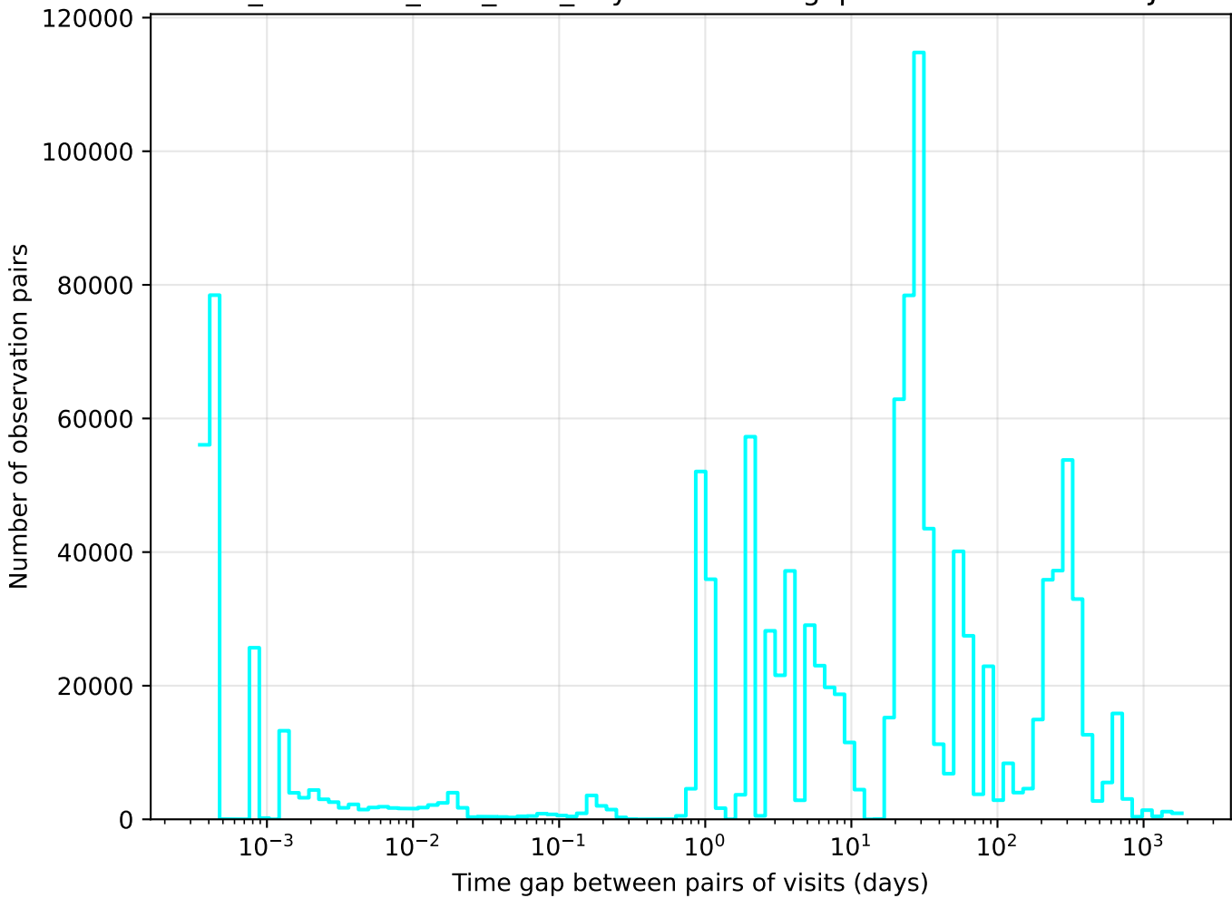
too_combined_s2.0_v3.4_10yrs u band: Tgaps observationStartMJD
