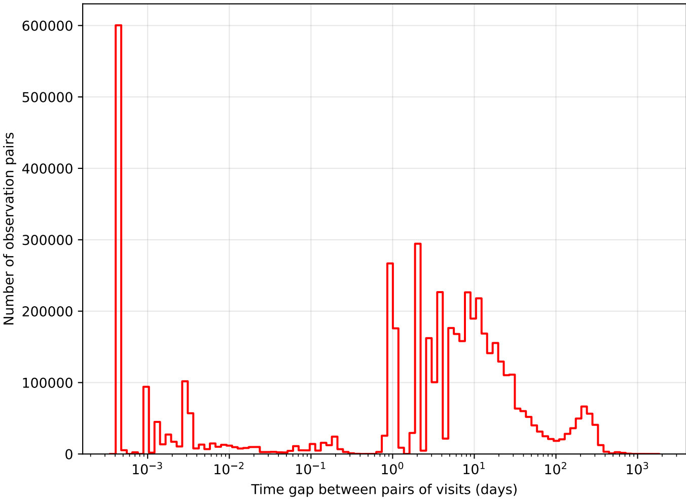
too_combined_s2.0_v3.4_10yrs i band: Tgaps observationStartMJD
