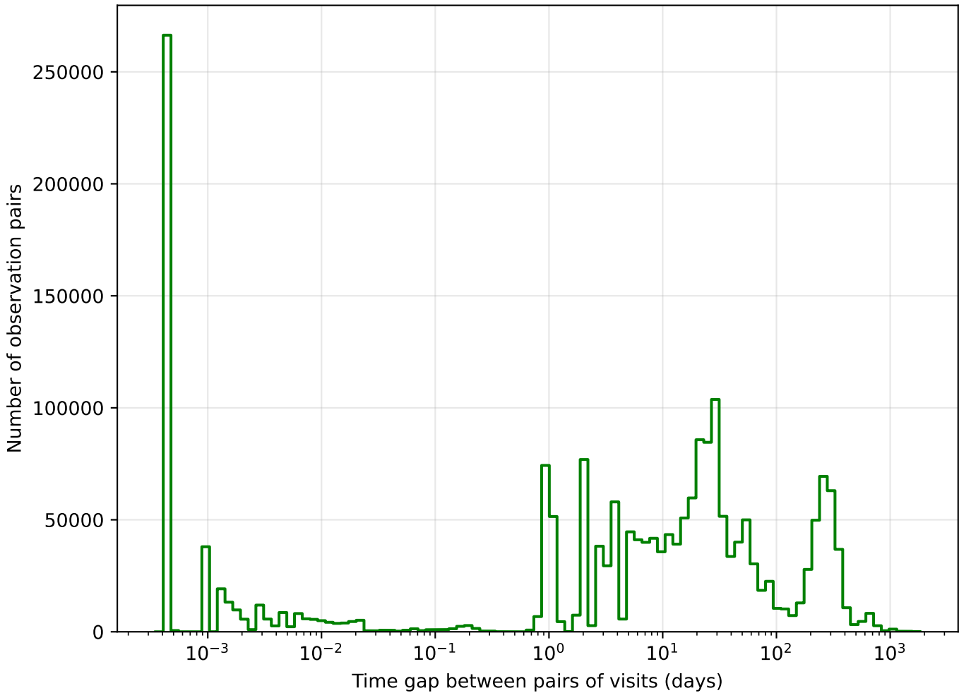
too_combined_s2.0_v3.4_10yrs g band: Tgaps observationStartMJD
