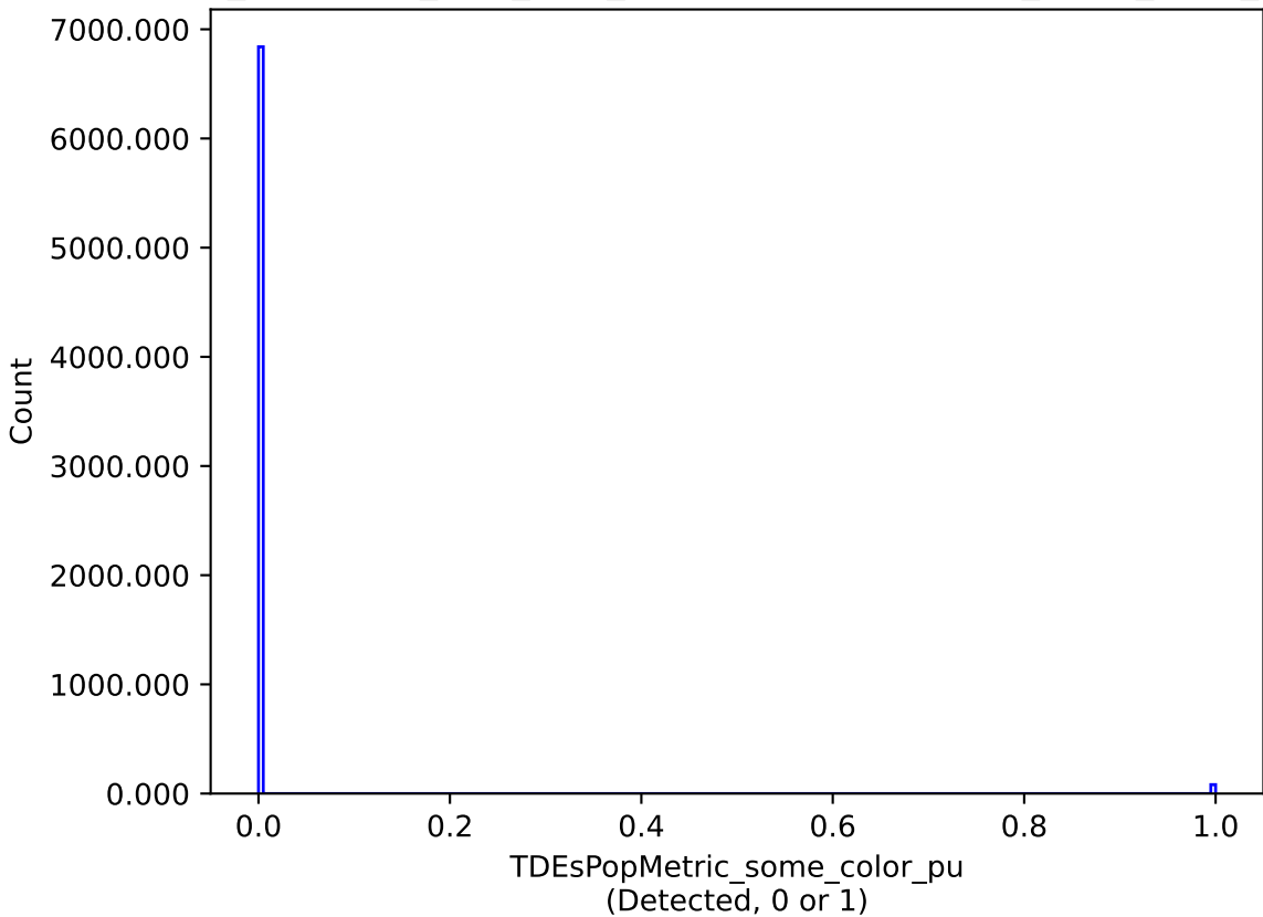
too_combined_s2.0_v3.4_10yrs : TDEsPopMetric_some_color_pu
