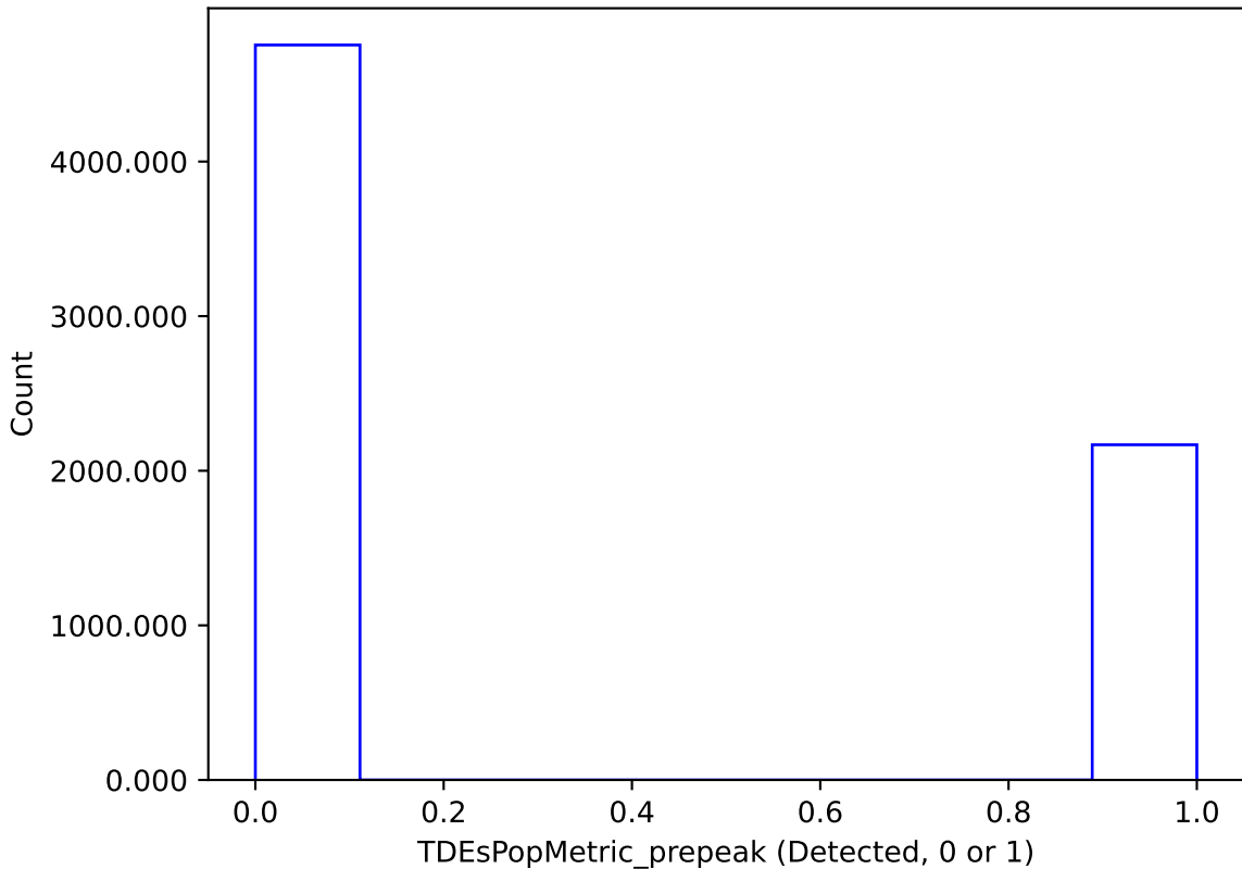
too_combined_s2.0_v3.4_10yrs : TDEsPopMetric_prepeak
