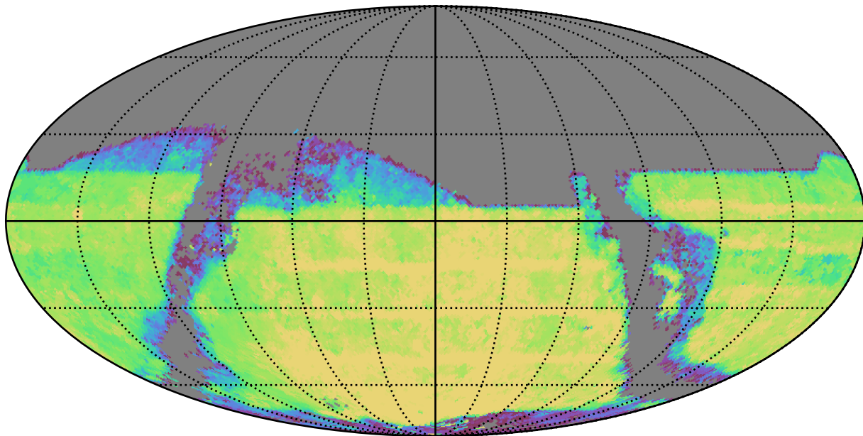
too_combined_s2.0_v3.4_10yrs : TDC_season
