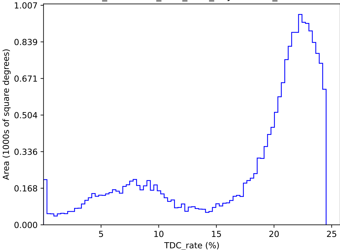
too_combined_s2.0_v3.4_10yrs : TDC_rate
