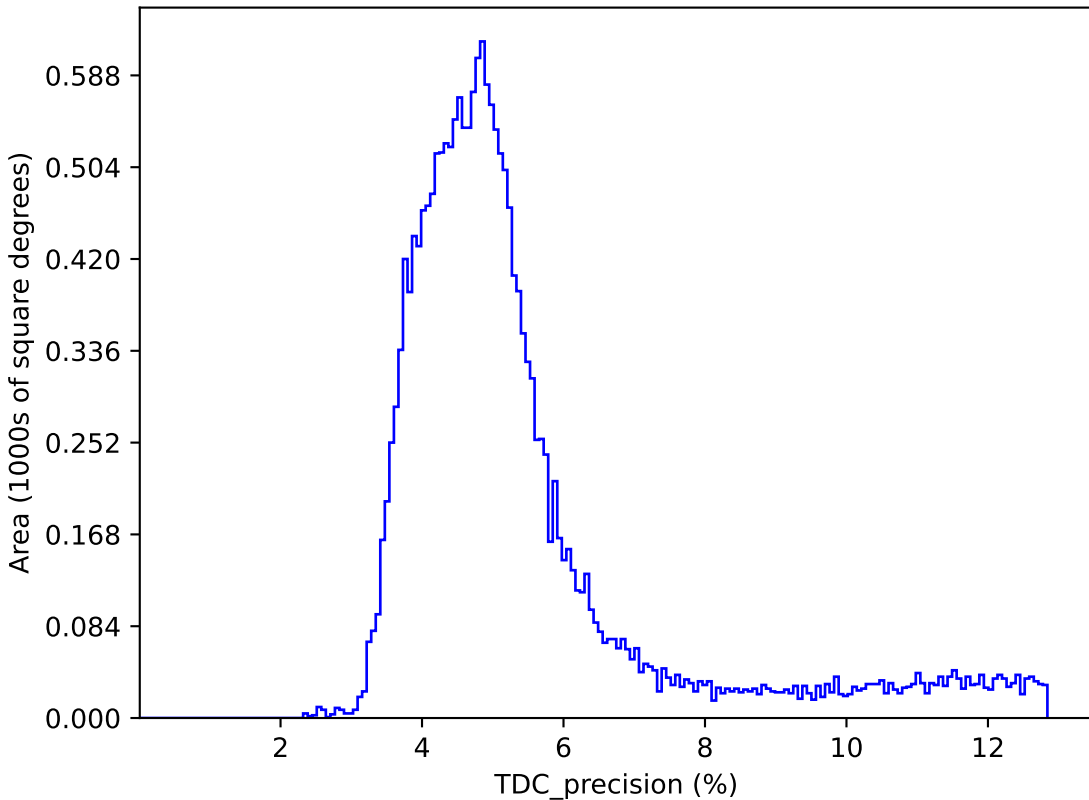
too_combined_s2.0_v3.4_10yrs : TDC_precision
