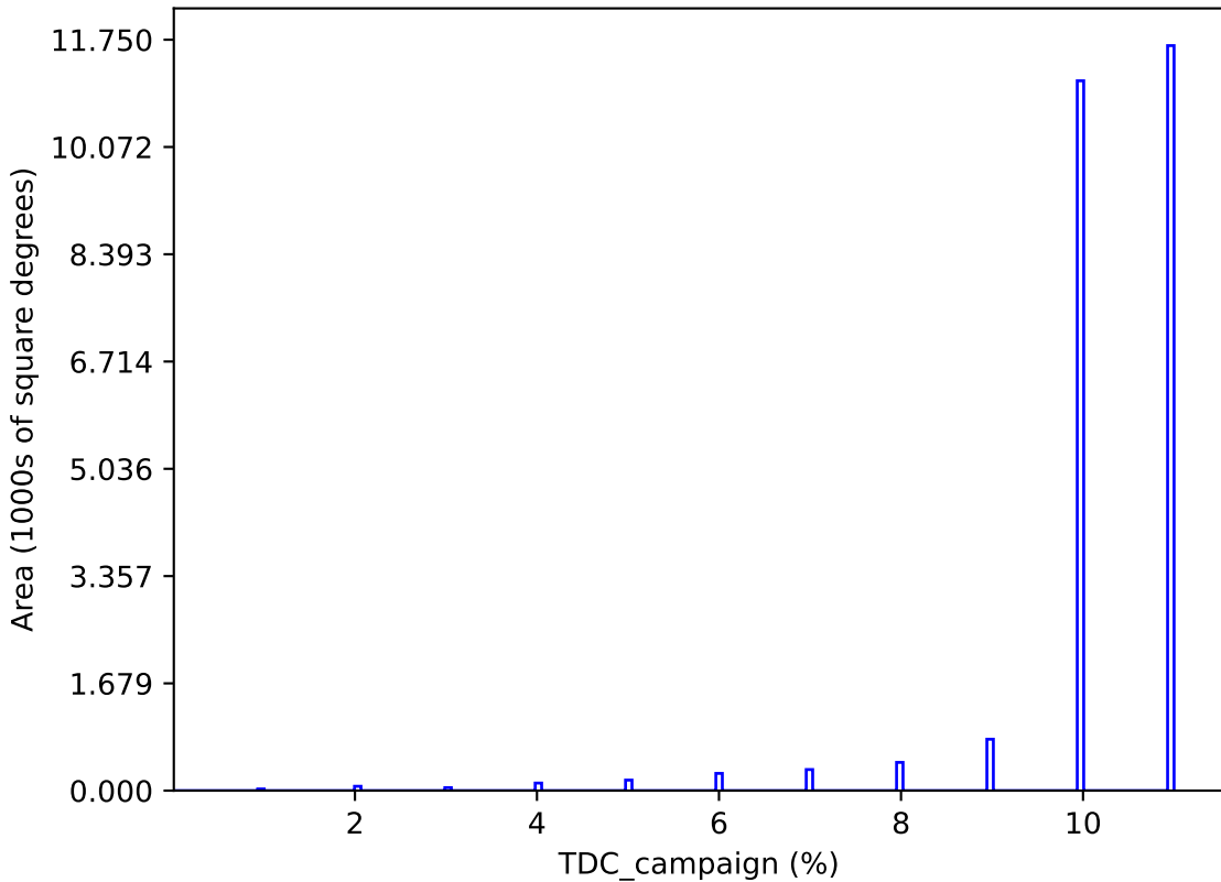
too_combined_s2.0_v3.4_10yrs : TDC_campaign
