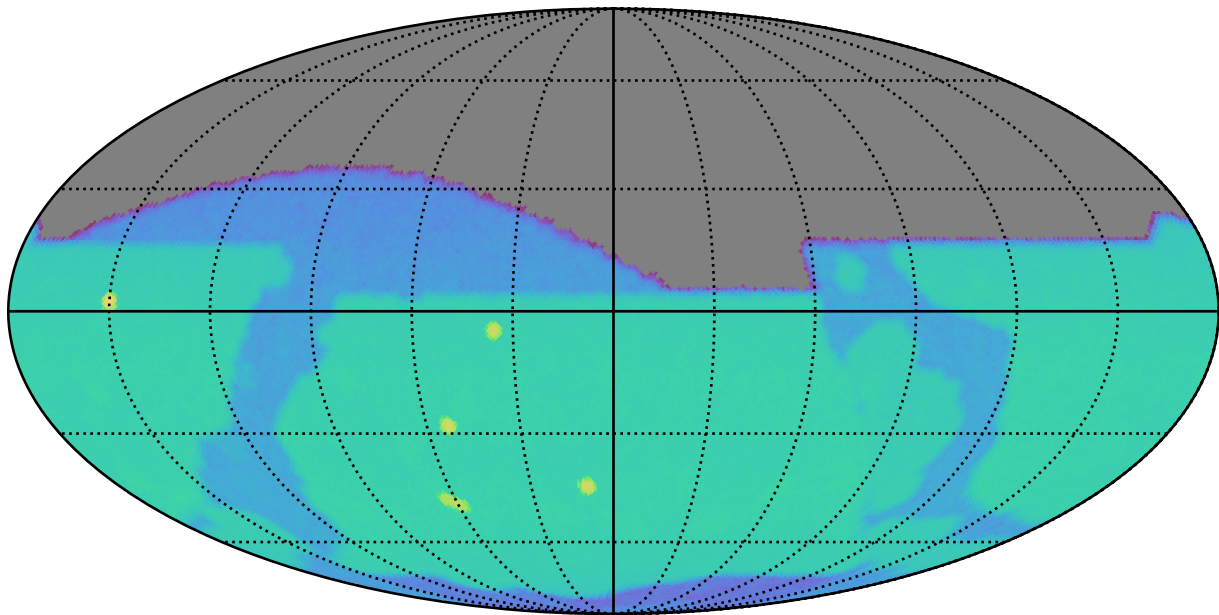
too_combined_s2.0_v3.4_10yrs z: SurfaceBrightLimit
