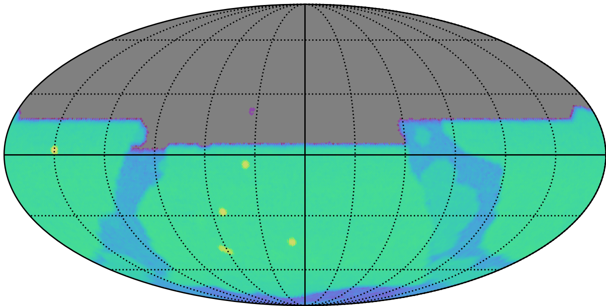
too_combined_s2.0_v3.4_10yrs y: SurfaceBrightLimit
