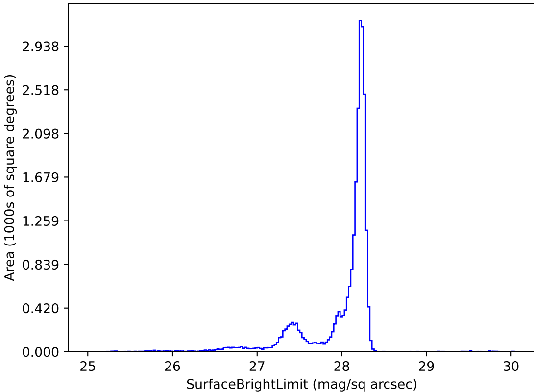
too_combined_s2.0_v3.4_10yrs y: SurfaceBrightLimit
