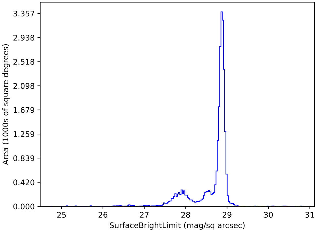
too_combined_s2.0_v3.4_10yrs u: SurfaceBrightLimit
