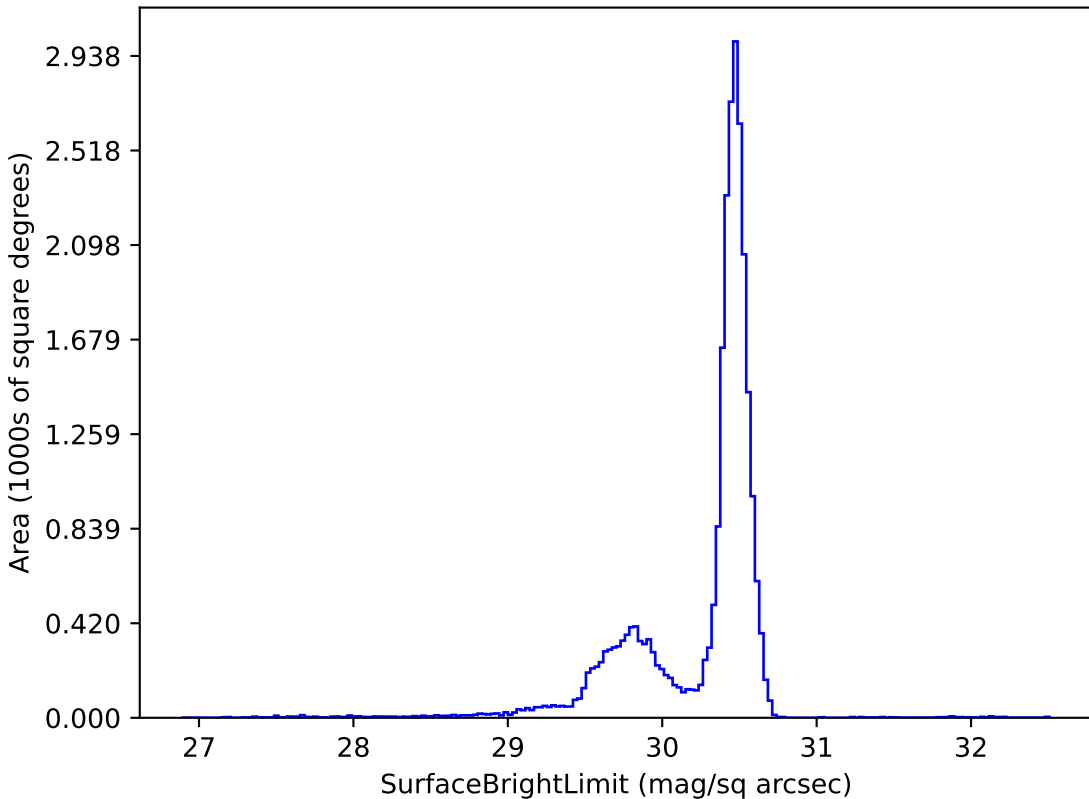
too_combined_s2.0_v3.4_10yrs r: SurfaceBrightLimit
