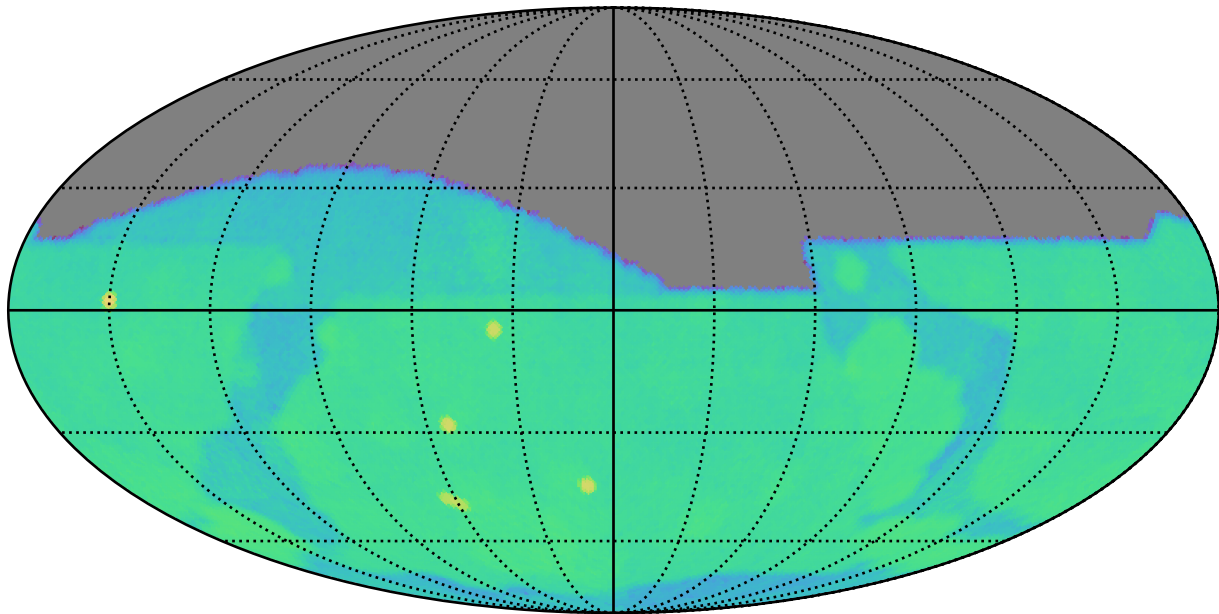
too_combined_s2.0_v3.4_10yrs g: SurfaceBrightLimit
