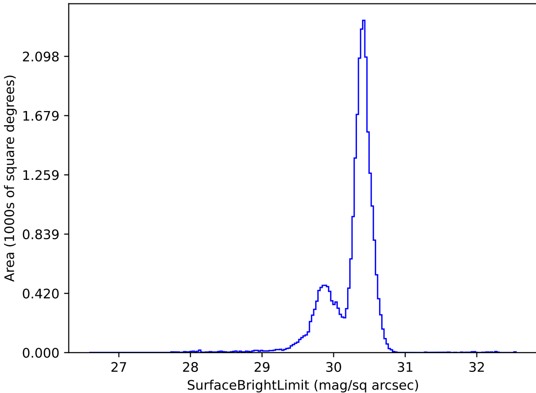
too_combined_s2.0_v3.4_10yrs g: SurfaceBrightLimit
