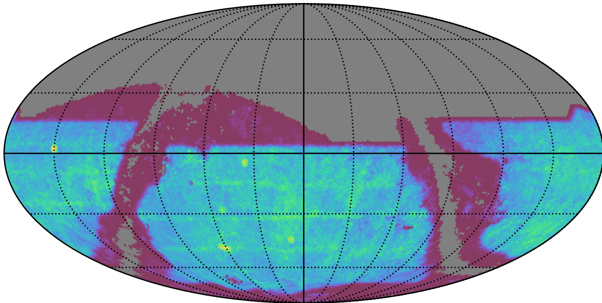
too_combined_s2.0_v3.4_10yrs : SNSLMetric
