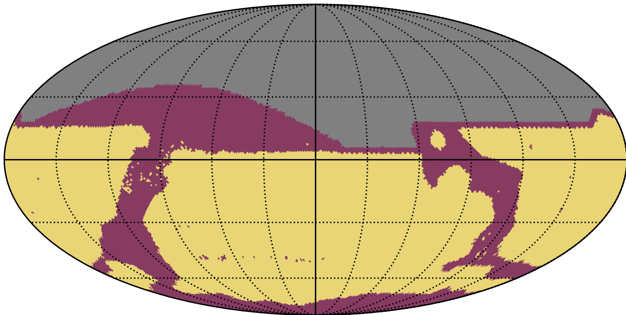
too_combined_s2.0_v3.4_10yrs : RapidRevisits
