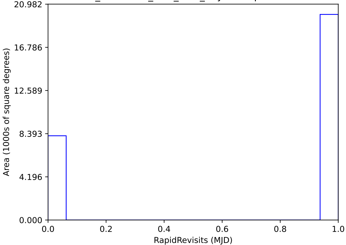
too_combined_s2.0_v3.4_10yrs : RapidRevisits
