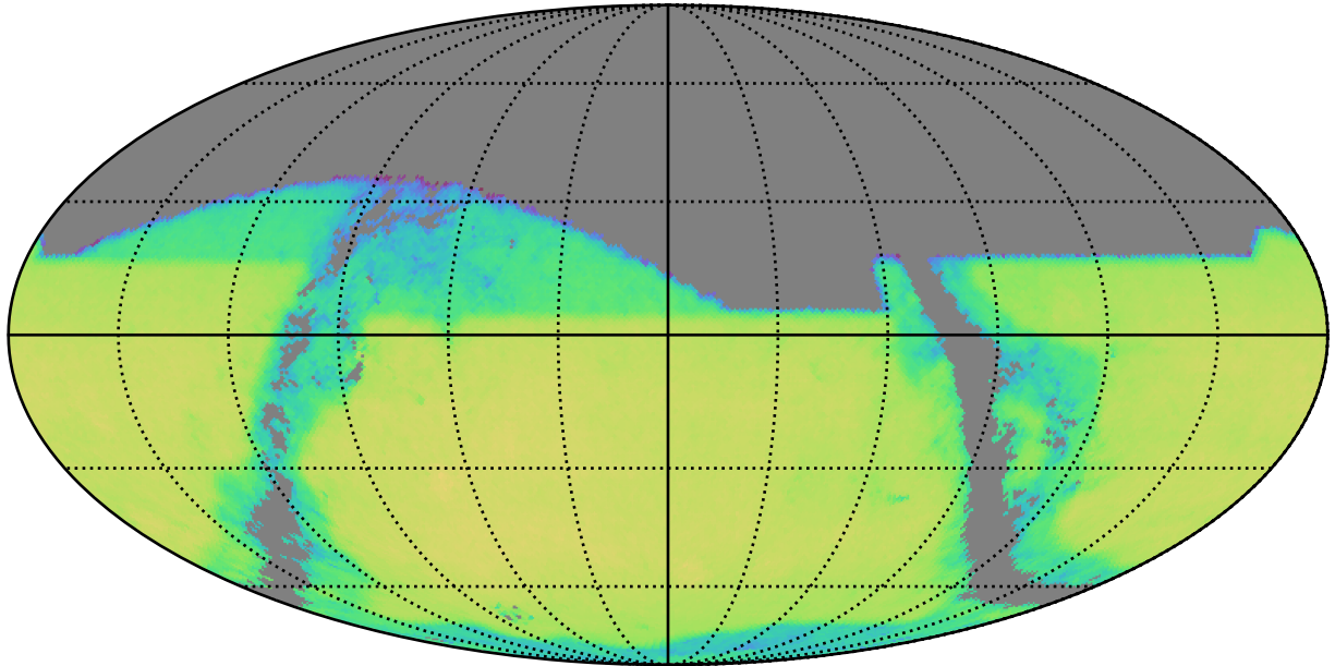
too_combined_s2.0_v3.4_10yrs z band and non-DD: QSONumberCountsMetric
