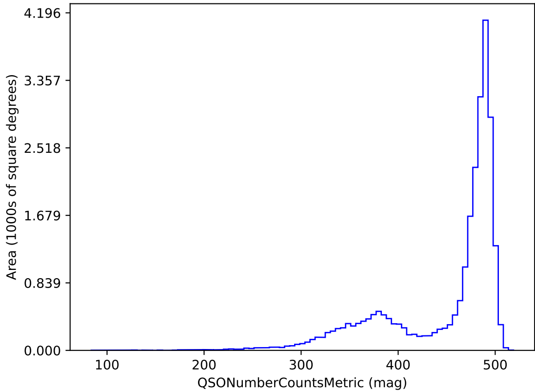
too_combined_s2.0_v3.4_10yrs z band and non-DD: QSONumberCountsMetric
