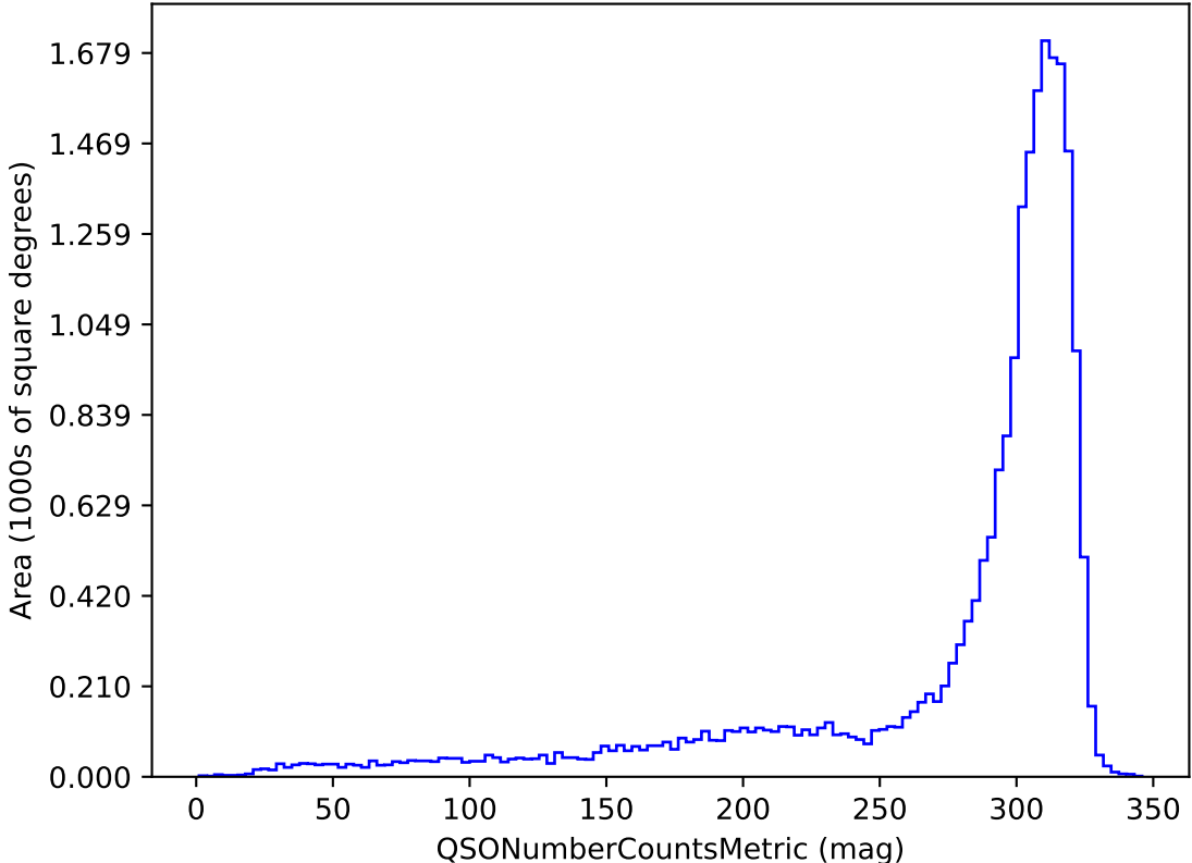
too_combined_s2.0_v3.4_10yrs u band and non-DD: QSONumberCountsMetric
