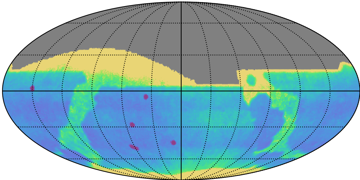
too_combined_s2.0_v3.4_10yrs : Proper Motion Uncert @ 24.0
