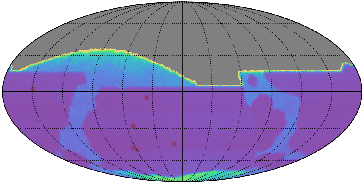
too_combined_s2.0_v3.4_10yrs : Proper Motion Uncert @ 20.5
