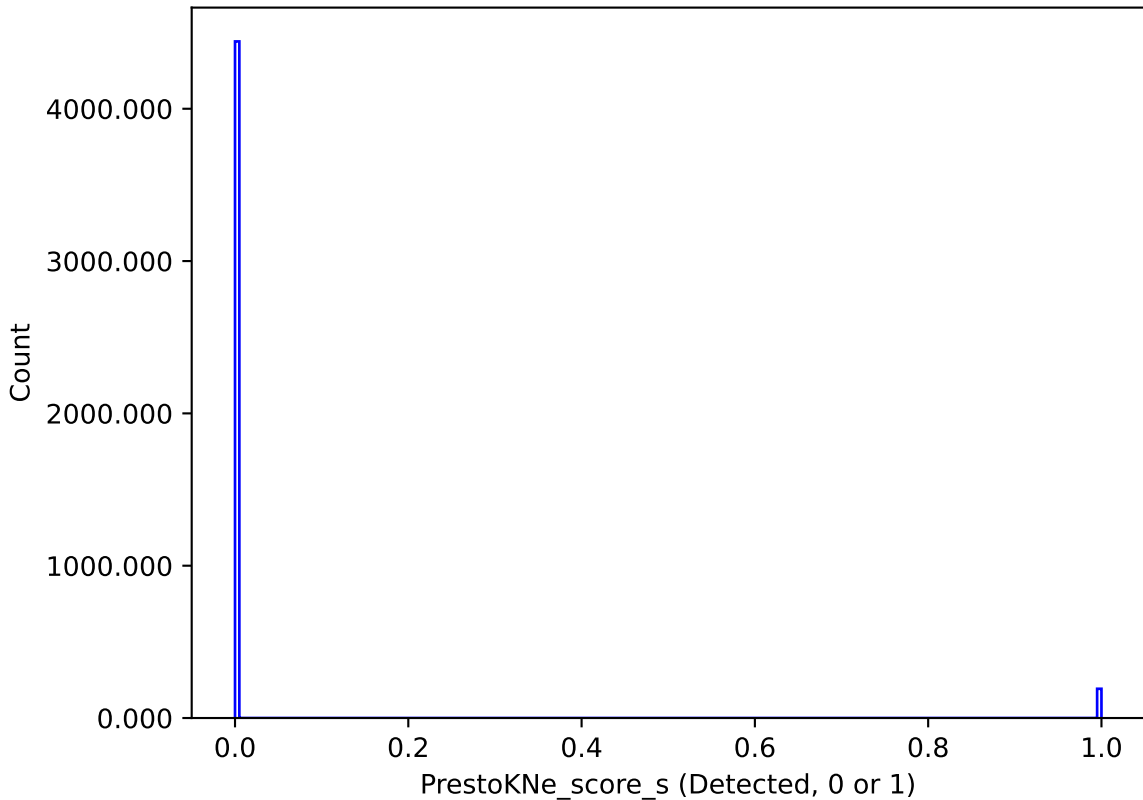
too_combined_s2.0_v3.4_10yrs : PrestoKNe_score_s
