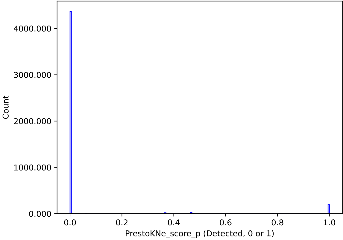
too_combined_s2.0_v3.4_10yrs : PrestoKNe_score_p
