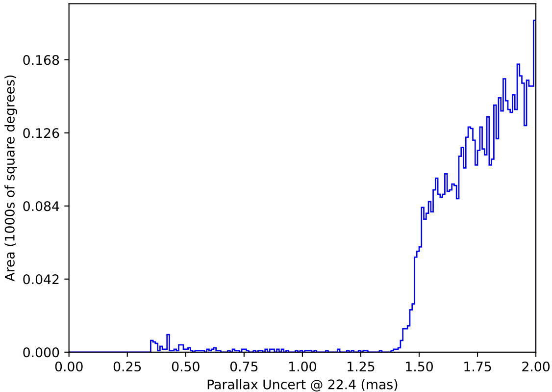
too_combined_s2.0_v3.4_10yrs : Parallax Uncert @ 22.4
