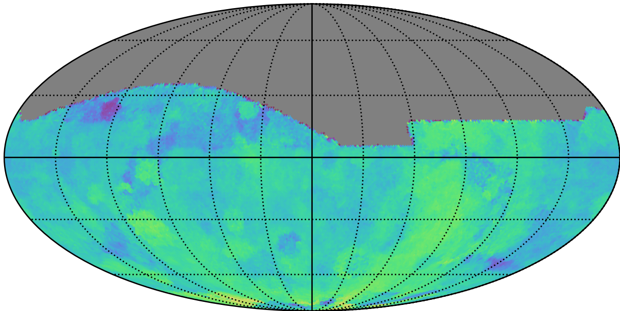
too_combined_s2.0_v3.4_10yrs : Parallax Coverage @ 24.0
