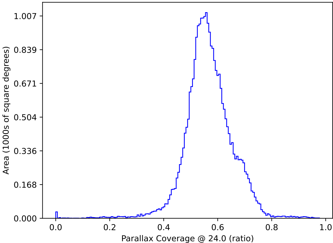
too_combined_s2.0_v3.4_10yrs : Parallax Coverage @ 24.0
