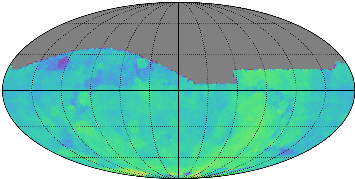
too_combined_s2.0_v3.4_10yrs : Parallax Coverage @ 22.4
