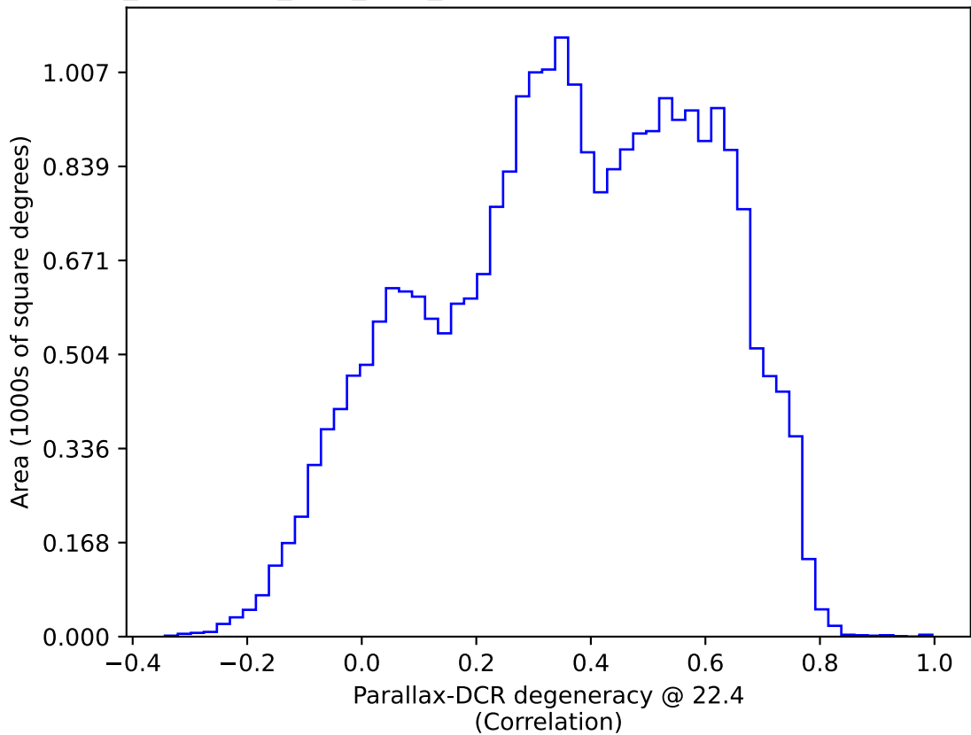
too_combined_s2.0_v3.4_10yrs : Parallax-DCR degeneracy @ 22.4
